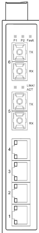
Front Panel of the 4-port 10/100TX + 2-port 100FX Industrial Switch
